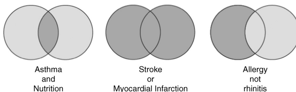
Figure 1 Boolean Operators
